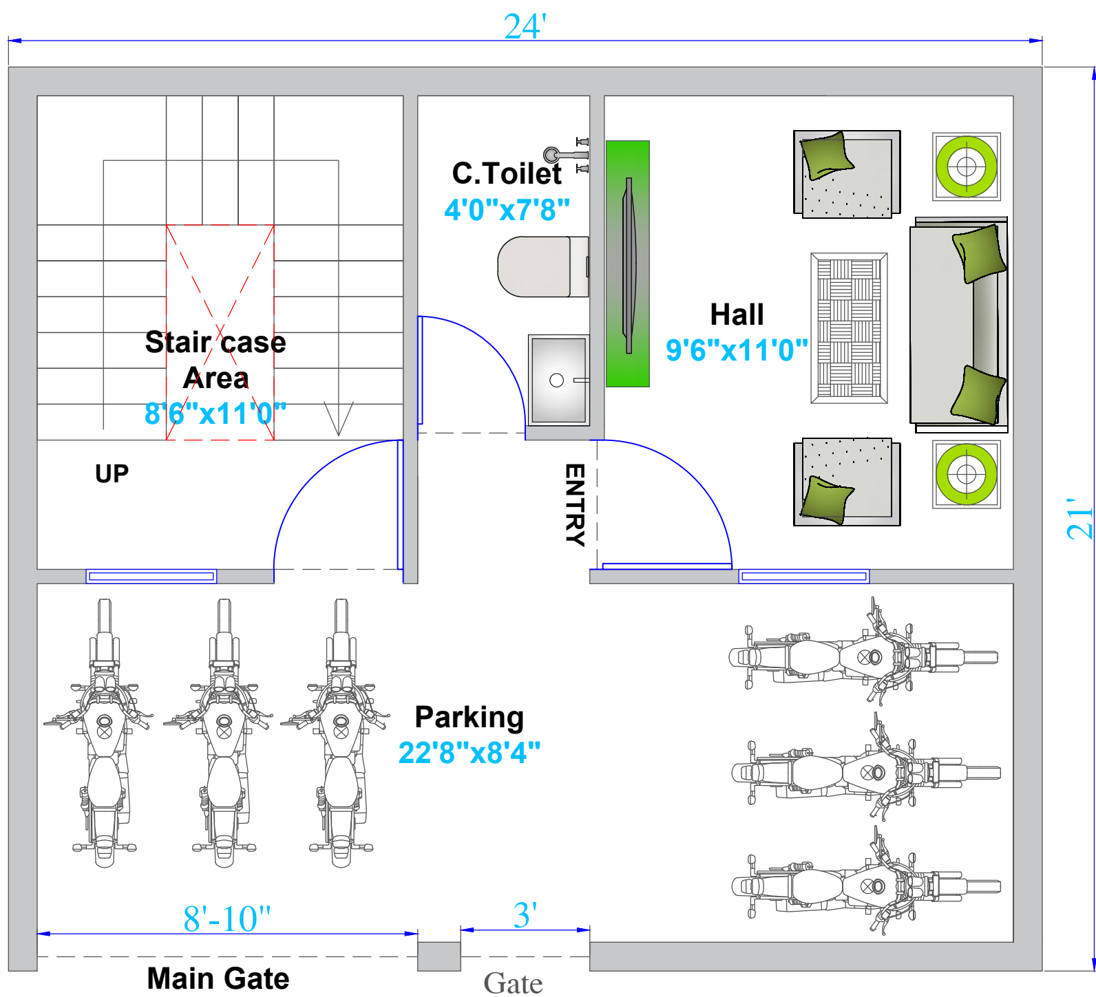
GROUND FLOOR
