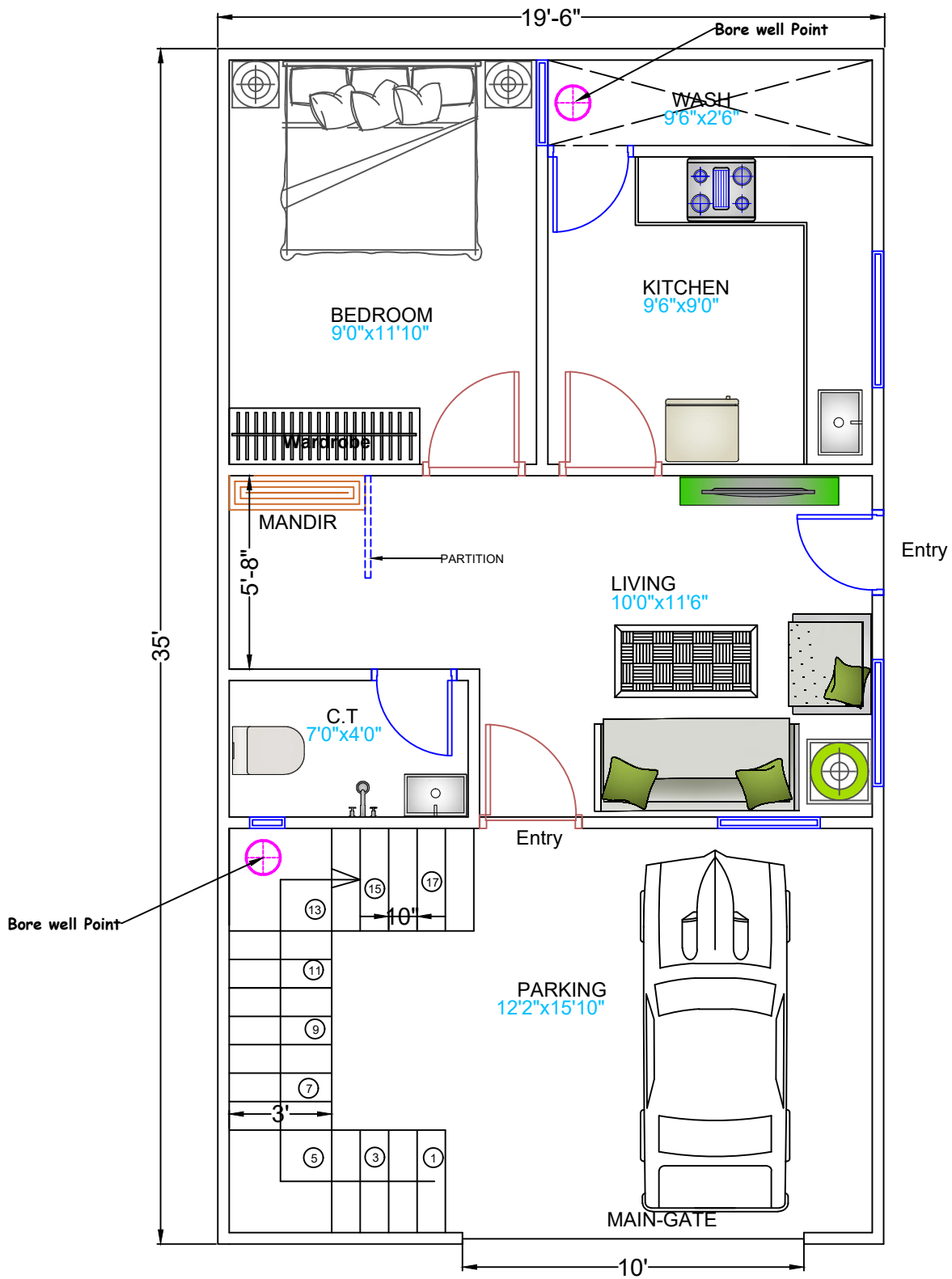
FINAL-GROUND FLOOR-WEST
